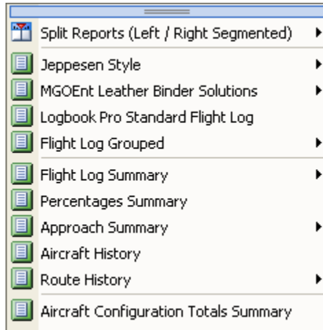
Figure 2. Detachable Menu
